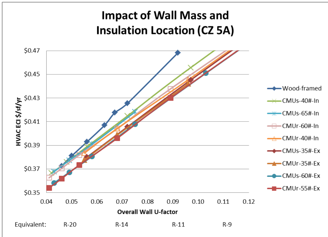
Figure 15. ECI vs. U-factor with Reduced-web CMU, Climate Zone 5A
