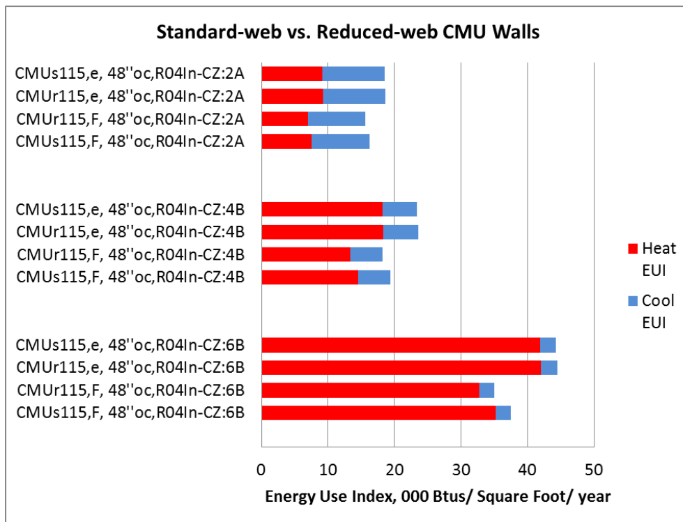
Figure 13. EUI for Standard vs. Reduced-Web CMU 18
