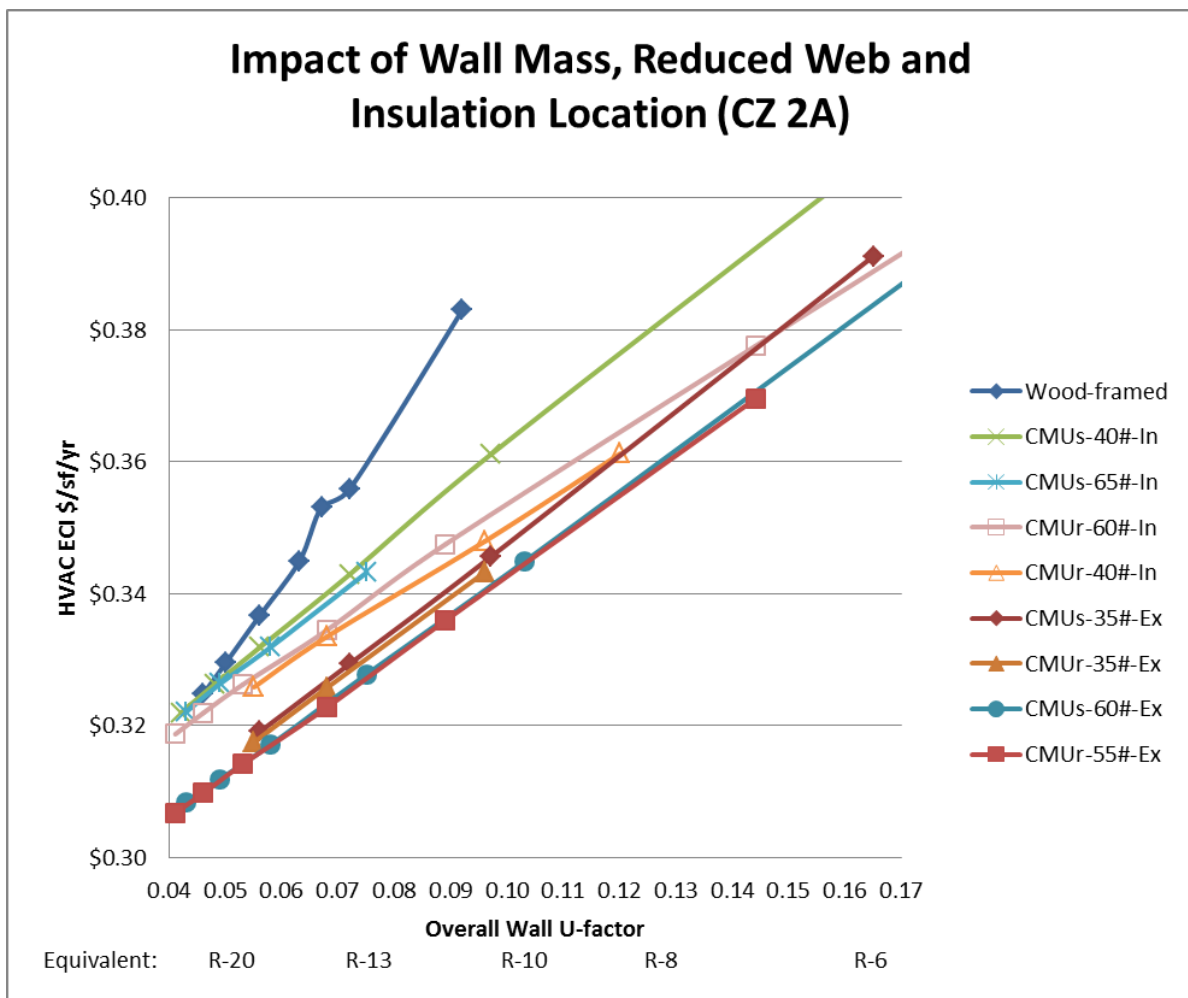
Figure 14. ECI vs. U-factor with Reduced-web CMU, Climate Zone 2A
